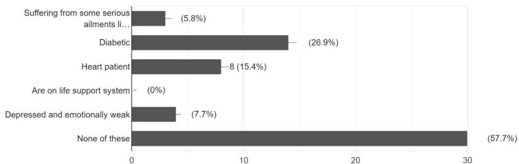
Fig. 2. Graphical Analysis of Survey Done
