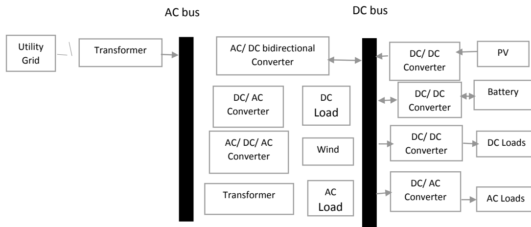
Fig. 4. Hybrid AC/DC Microgrid
