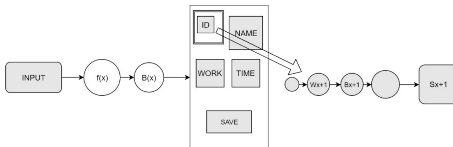
Fig 5. A diagram which shows how CNN model works to find the proper template for the user
