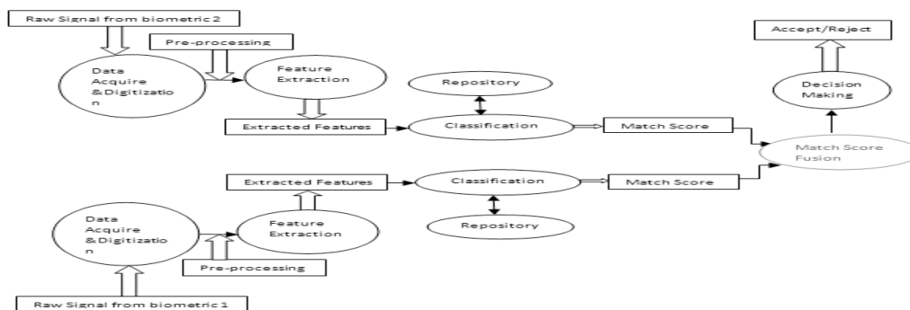
Fig. 5. Fusion at classification level
