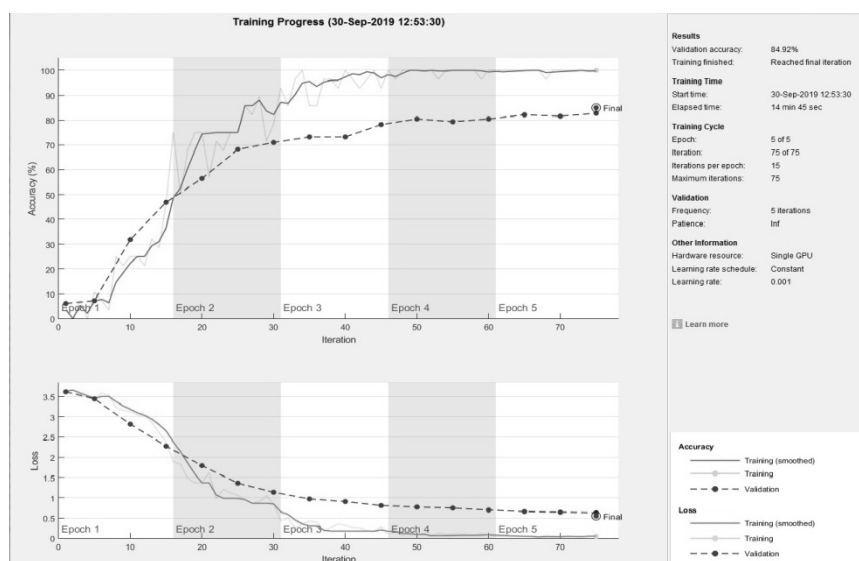
Fig. 6. Training and Loss curves of Fish_Net method for QUT dataset
