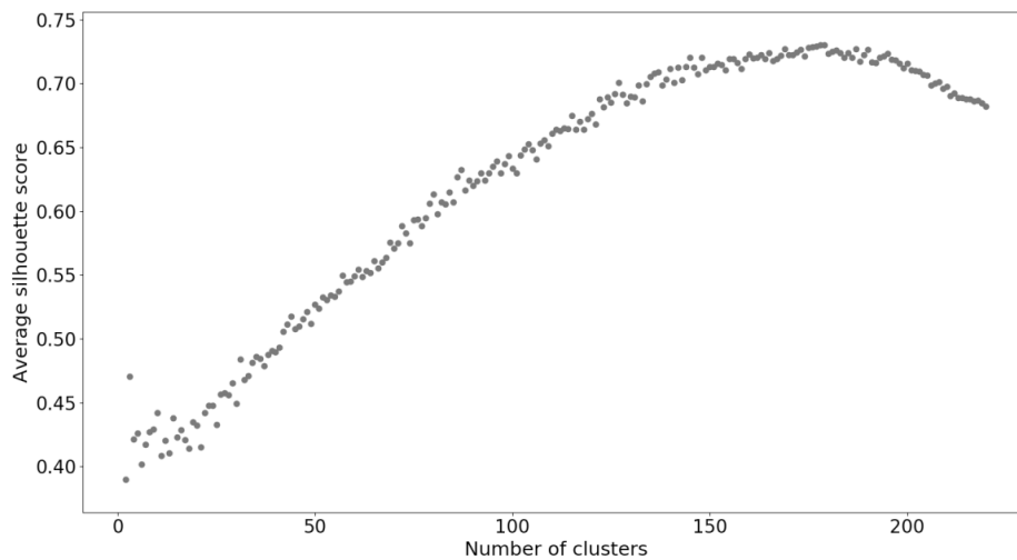
Fig. 1. Average Silhouette score for different number of clusters for duration vector of length 5.
