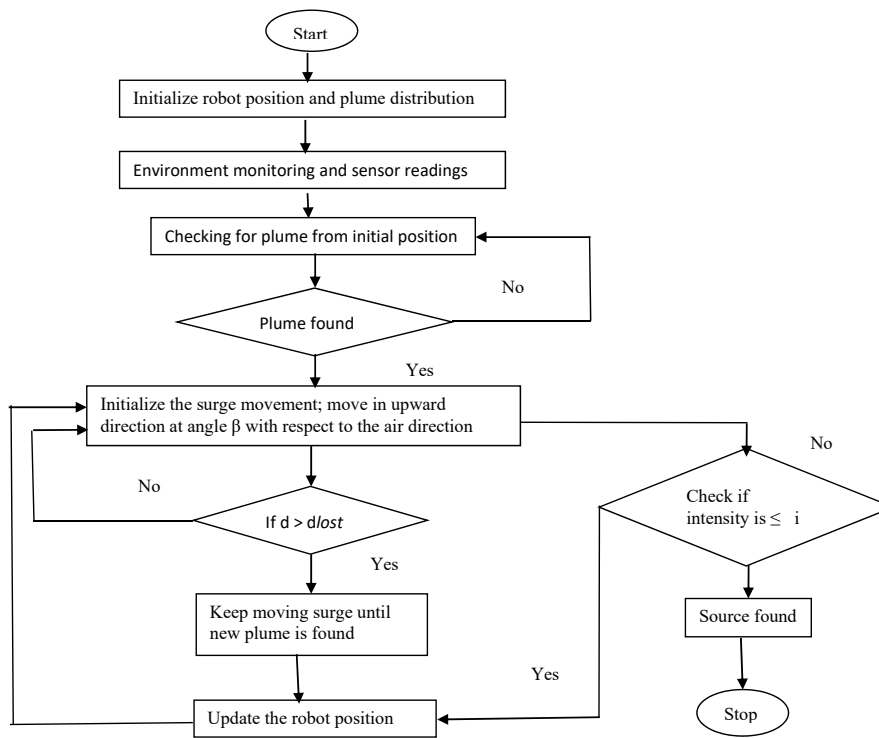
Fig. 1. Flowchart of Casting method for gas leakage source localization by a mobile robot
