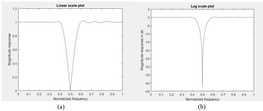
Fig. 2. (a) Magnitude response of LPF of 20 th order (b) Magnitude response in dB scale
