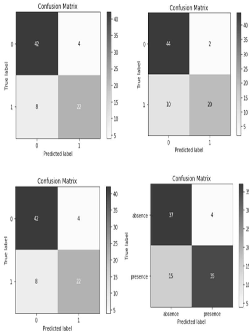
Fig. 3. Confusion Matrix of support vector matrix (SVM), Artificial Neural Network (ANN), Random Forest(RF) and XGBoost
