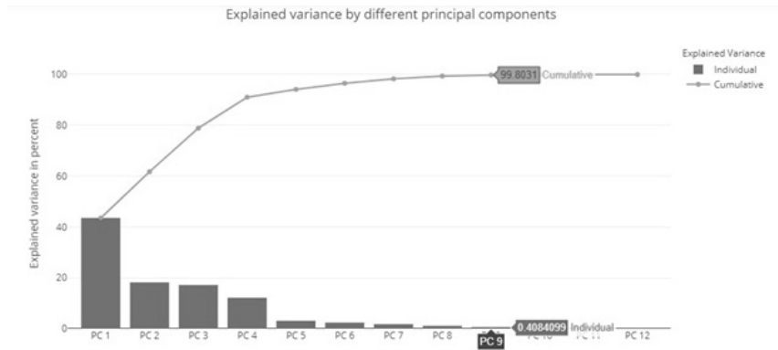
Fig. 2. Principal Component Analysis Graph representing the variance explained by the components
