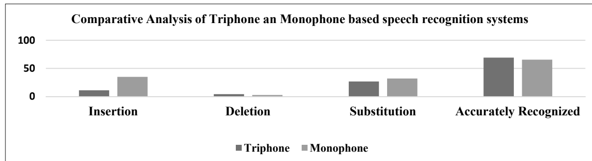
Fig. 3. Comparative analysis of Monophones and Triphones based continuous Hindi Speech Recognition systems
