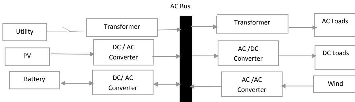
Fig. 2. AC Microgrid architecture
