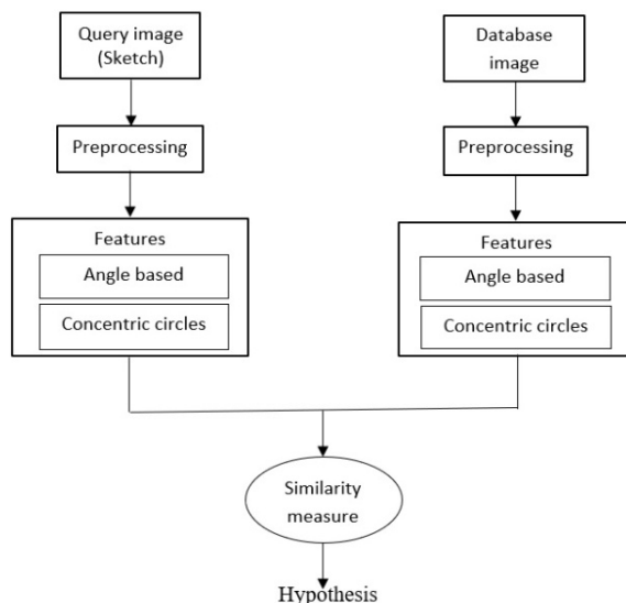
Fig. 1. Propose architecture of Sketch Based Image Retrieval
