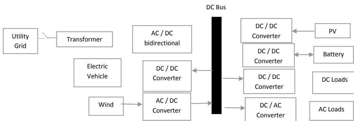
Fig. 3. DC Microgrid architecture
