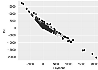
Fig. 5. DBSCAN clusters
