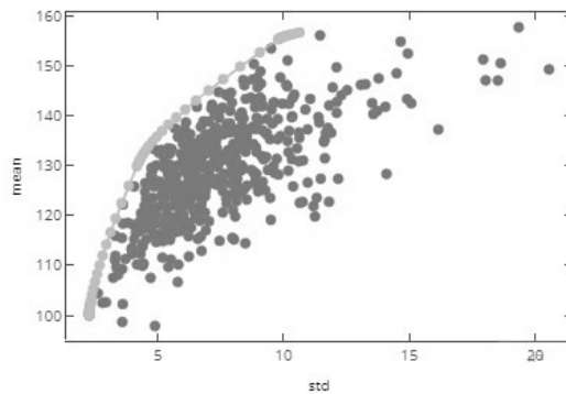
Fig. 5. Return vs. Risk Curve
