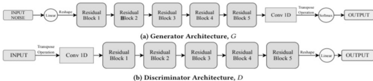
Fig. 1. Passgan architecture
