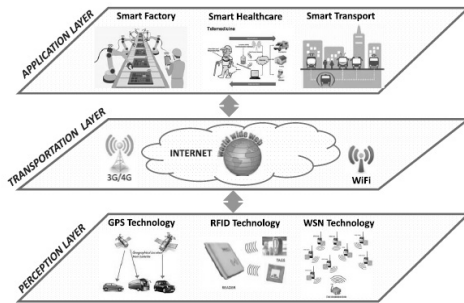
Fig. 2. IoT system Model [5]
