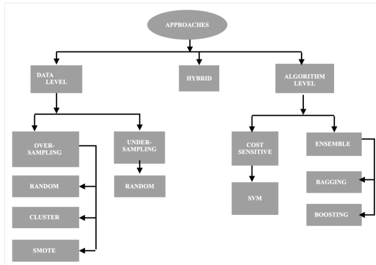
Fig. 1. Approaches to solve Imbalance Classification Problem
