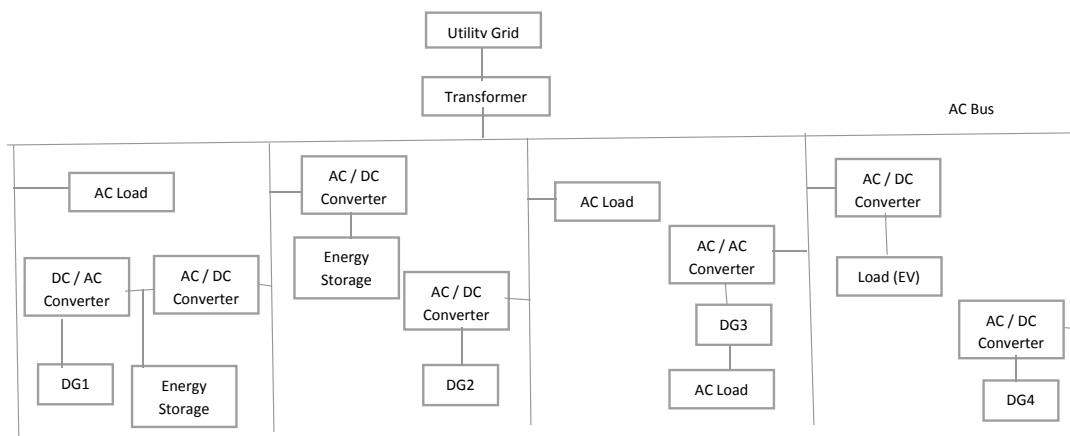
Fig. 1. Architecture of a Microgrid
