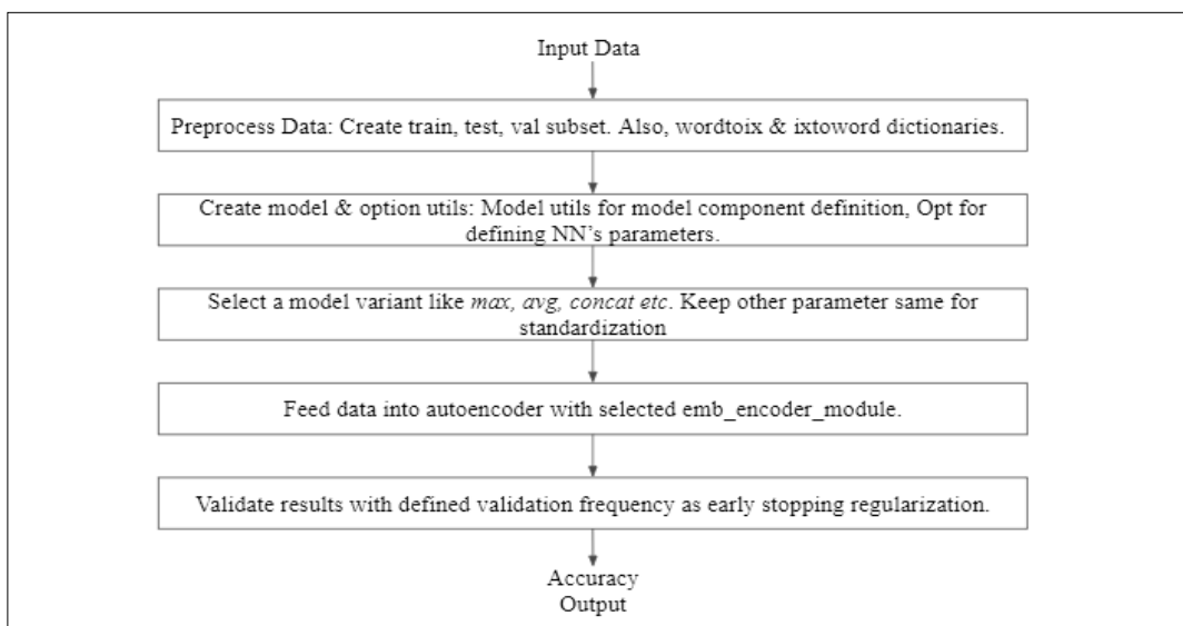
Fig. 1. Explanation of Simple Word Embedding Model in form of flowchart
