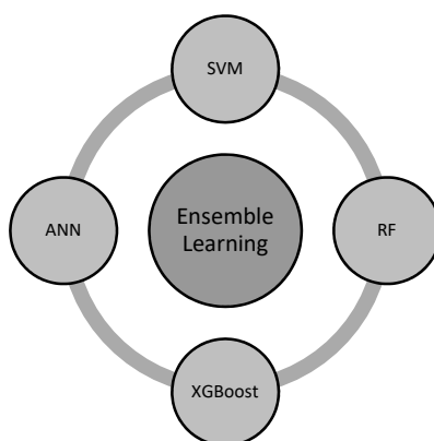
Fig. 1. Ensemble Model
