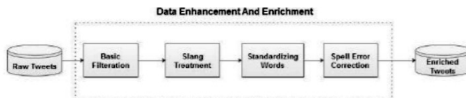
Fig. 2. Framework of Data Enhancement and Enrichment
